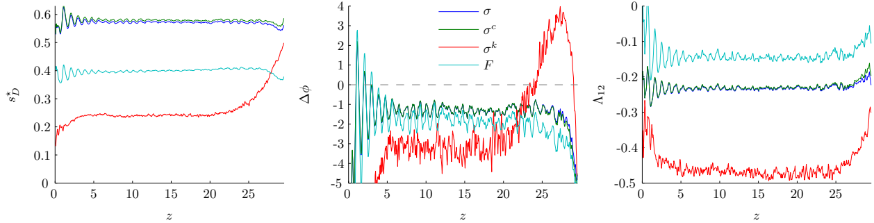
FIG. 12. Decomposition of the symmetric traceless parts of the total, contact and kinetic stresses and of the fabric tensor, into magnitude s_D^* (left), angular deviation \Delta\phi (center) and eigenvalue ratio \Lambda_{12} (right). Data are taken for N = 6000 , \theta = 28^\circ , w = 0.05 .
