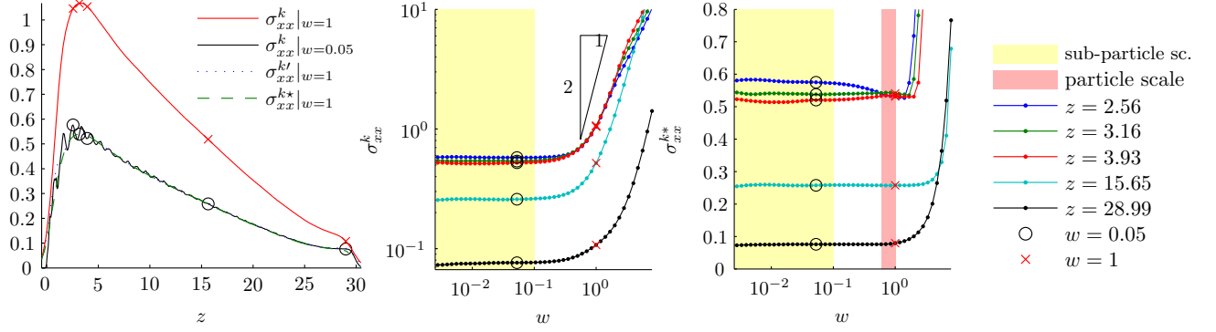
FIG. 4. Left: Kinetic stress component \sigma_{xx}^k as a function of height for w = 0.05 and w = 1 , as well as the reduced kinetic stress components \sigma_{xx}^{k'} and \sigma_{xx}^{k*} for w = 1 . Kinetic stress component \sigma_{xx}^k (middle) and scale-corrected kinetic stress component \sigma_{xx}^{k*} (right) at selected heights as a function of the coarse-graining width w . Circles and crosses denote the values at the selected heights for w = 0.05 and w = 1 , respectively.
