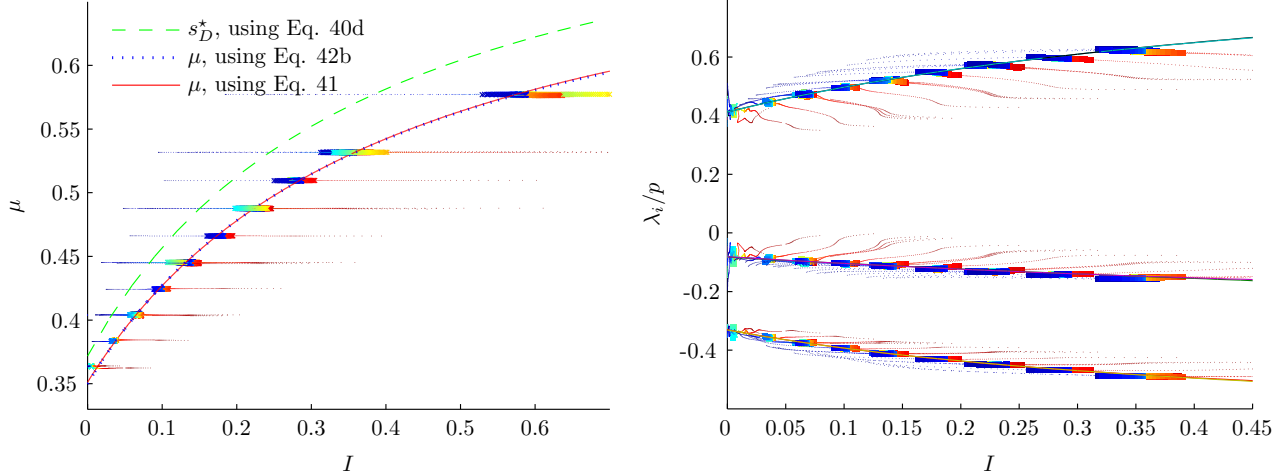
FIG. 11. Friction \mu = -\sigma_{xz}/\sigma_{zz} ( left panel ) and eigenvalues of the deviatoric stress \lambda_i scaled by the pressure p ( right panel ), plotted as function of the inertial number I . Data from various simulations with 4000 \leq N \leq 8000 , 20^\circ \leq \theta \leq 28^\circ , and w = 1 , using the reduced kinetic stress (34). The solid lines in each plot are the predictions for \mu and \lambda_i/p , (42), from the (anisotropic) constitutive equations, (40). The dotted line (blue online) in the left panel is the prediction according to the (isotropic) \mu(I) rheology, (41), the dashed line (green online) is the objective friction s_D^* , see (40d).
