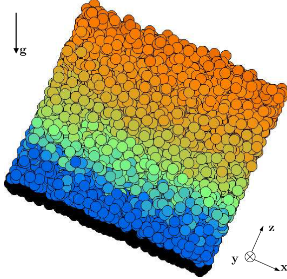
FIG. 1. DPM simulation for N = 3500 and inclination \theta = 24^\circ at time t = 2000 ; gravity direction \mathbf{g} as indicated. The domain is periodic in x - and y -directions. In the z -direction, fixed particles (black) form a rough base while the surface is unconstrained. Shades/colors indicate speed, from darkest gray (blue online) through light gray (green/yellow online) to mid-gray (orange online) as z increases.
