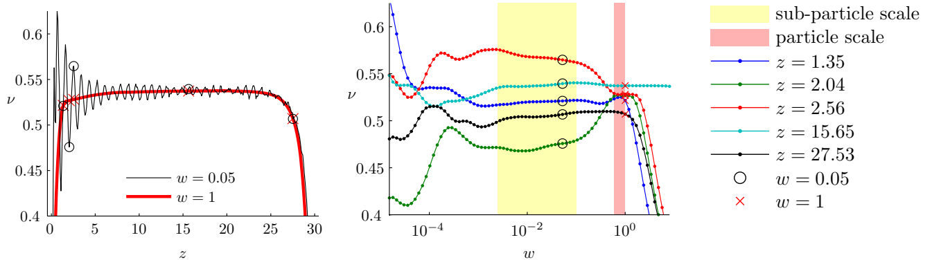
FIG. 3. Left: Volume fraction as a function of height for w = 0.05 and w = 1 . Right: Volume fraction at selected heights as a function of the coarse-graining width w . Circles and crosses in both figures denote the density at the selected heights for w = 0.05 and w = 1 , respectively. Data taken for N = 6000 , \theta = 28^\circ .
