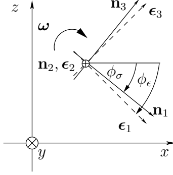
FIG. 2. Sketch of the eigendirections \mathbf{n}_i of the deviatoric stress tensor, the eigendirections \epsilon_i of the strain rate tensor, and the angles \phi_\sigma and \phi_\epsilon between the x -axis and the largest (smallest) principal direction of the deviatoric stress (deviatoric strain rate) tensor.
