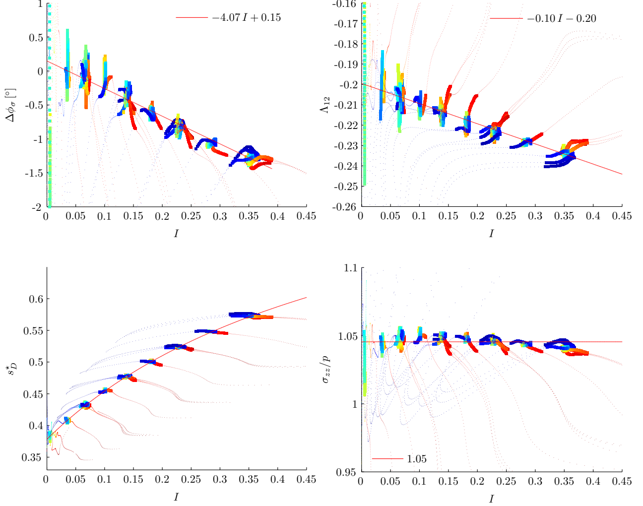
FIG. 10. The four objective variables that describe the stress tensor, one for isotropic pressure and three for the deviatoric stress, are plotted against the inertial number I . Large markers denote bulk values, while small dots denote base and surface values. Shade/color indicates relative height \hat{z} (see figure 8). Lines indicate fits to the bulk data as specified in the insets. Top left: Angular deviation of the deviatoric stress from collinearity with the strain rate tensor, \Delta\phi , with linear fit (40b). Bottom left: Magnitude of the deviatoric stress ratio, s_D^* , with the line a fit to the bulk data according to equation (40d). Top right: Ratio of eigenvalues \Lambda_{12} with linear fit (40c). Bottom right: Ratio of pressure p and confining stress \sigma_{zz} , with constant fit. Data are from steady simulations in the parameter range 4000 \leq N \leq 8000 , 20^\circ \leq \theta \leq 28^\circ , with coarse graining width w = 1 , using the reduced kinetic stress (34).
