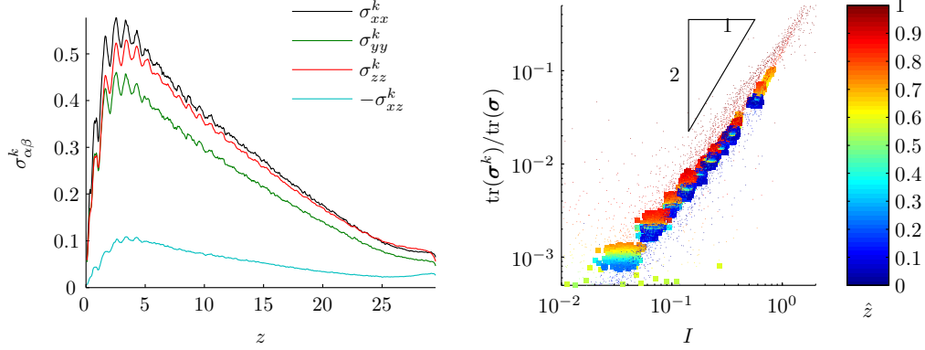
FIG. 8. Left: Kinetic stress components \sigma_{\alpha\beta}^k for N = 6000 , \theta = 28^\circ , w = 0.05 . Components not shown are nearly zero. Right: Ratio of total kinetic pressure to total pressure, \frac{\text{tr}(\sigma^k)}{\text{tr}(\sigma)} , as a function of inertial number for all data 4000 \leq N \leq 8000 , 20^\circ \leq \theta \leq 30^\circ , w = 0.05 . Shade/color indicates the relative height, \hat{z} = z/h , from darkest gray (blue online) at the bottom ( \hat{z} = 0 ) to light gray (green/yellow online) to mid-gray (red online) at the surface ( \hat{z} = 1 ). For the height definition, see Weinhart et al. 37
